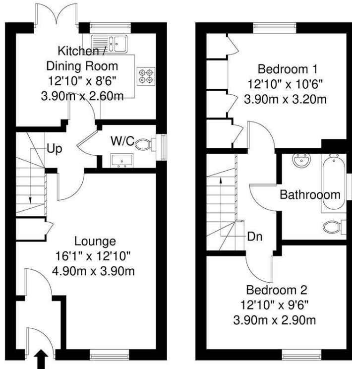
GROUND FLOOR 34.3 sq m / 369 sq ft
